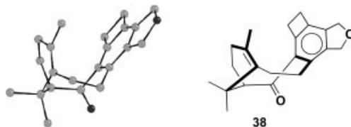
Figure 2. ORTEP representation of the cycloadduct 38 .
