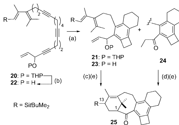
Scheme 8. (a) 5 mol-% [CpCo(CO) 2 ], xylenes, Δ, hv; (b) cat. PTSA, MeOH, quantitative; (c) IBX, DMSO, room temp., 76%; (d) 1. LDA, PhSeBr, THF, 2. NaIO 4 , NaHCO 3 , MeOH/H 2 O, 81%; (e) Et 2 O·BF 3 , CHCl 3 , –78 °C, 95%.
