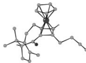
Figure 1. ORTEP representation of complex 11 .
